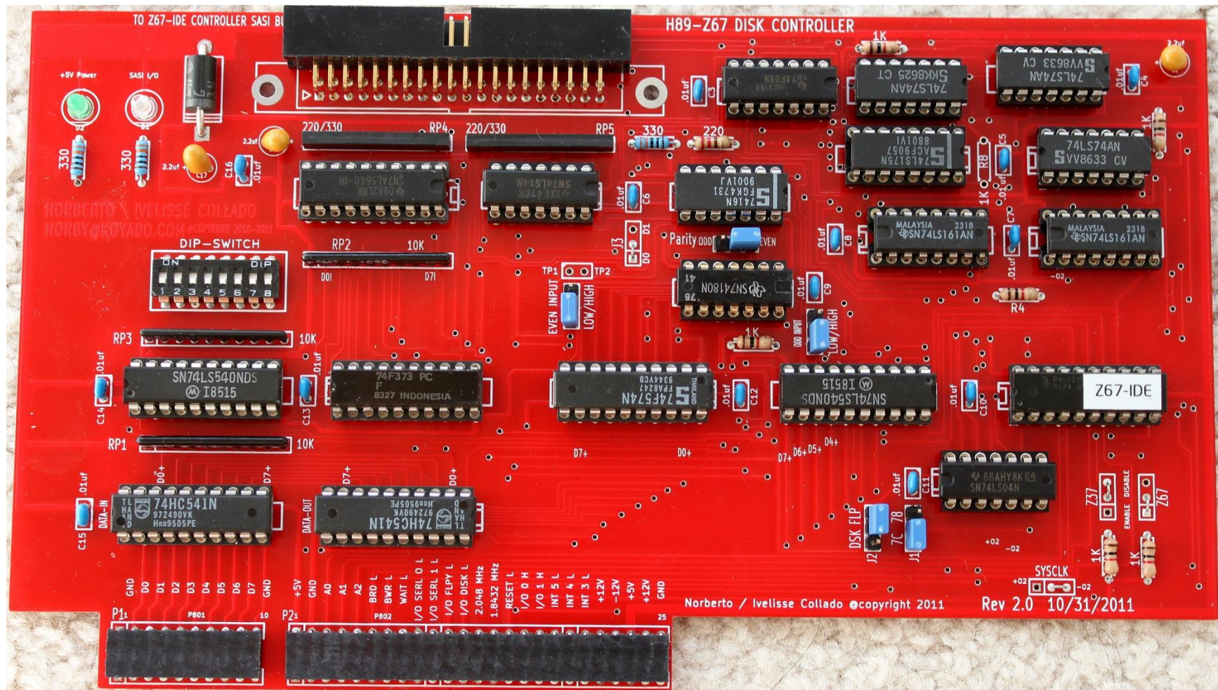
H89-Z67 Board
