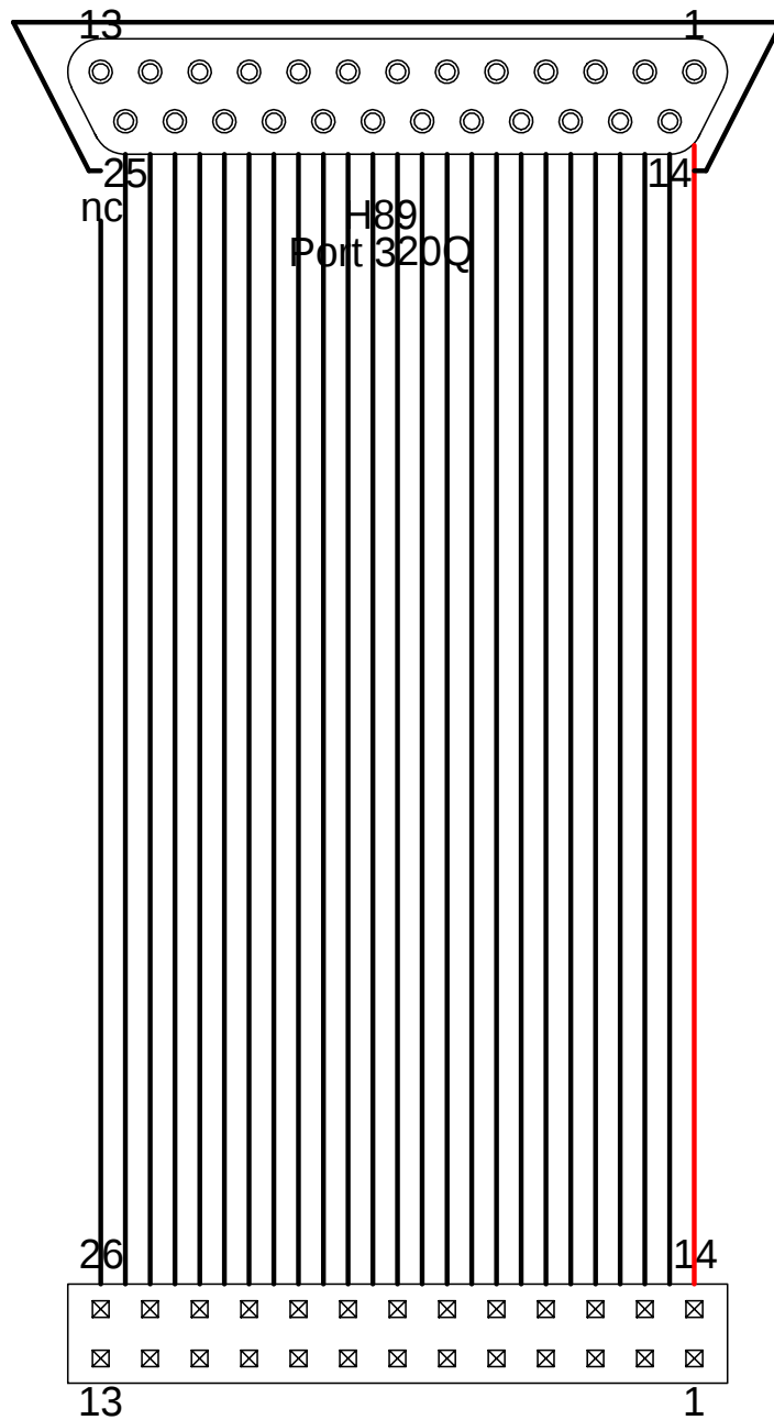
SCS Card 26 Pin
