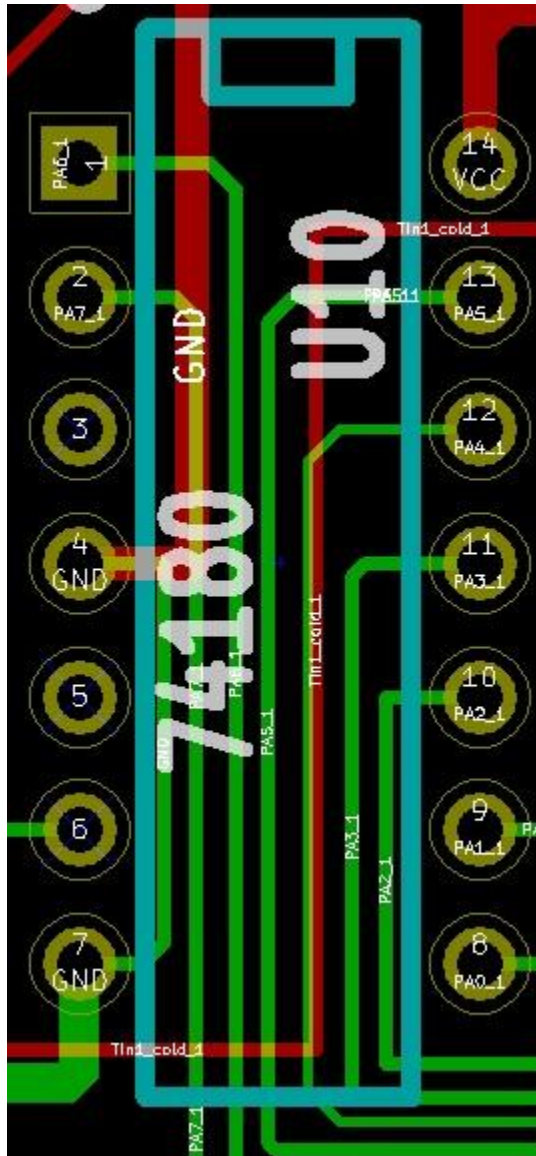
Board 74180 layout (pin6):
